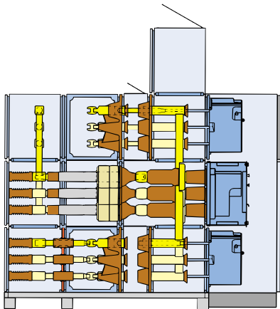
2000 A sectionalizer panel.
